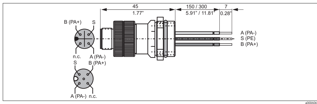
Fig. 16: M-12 plug with socket
