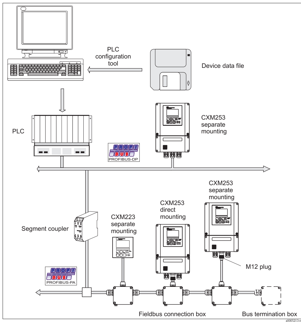
Fig. 15: Instrumentation overview Liquisys M CXM2x3
