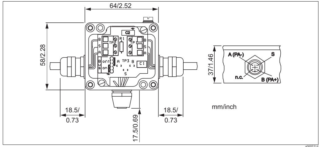
Fig. 17: Fieldbus connection box for PA
