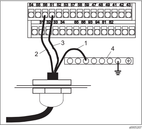
Fig. 9: Bus cable connection CLM253 conductive
