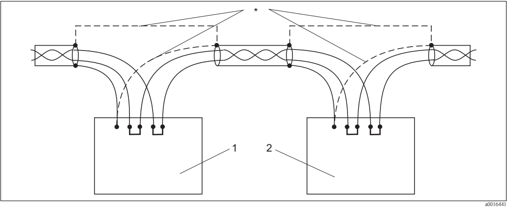
Fig. 11: Connection of several panel mounted instruments
