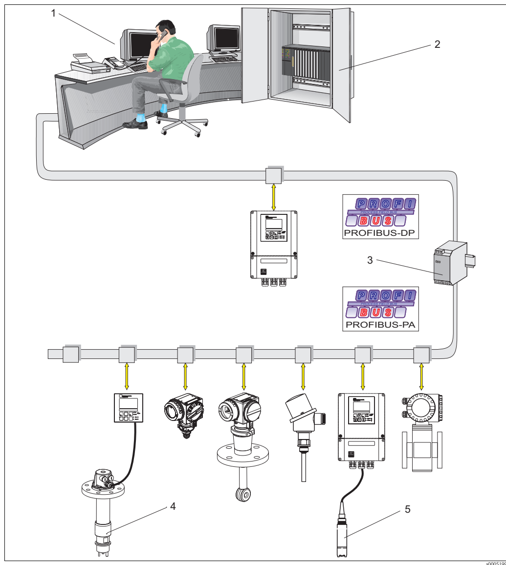
Fig. 1: Measuring system with PROFIBUS interface
