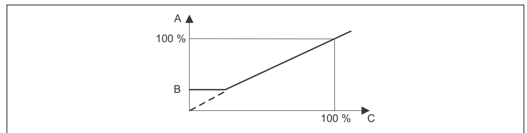
30 Control characteristic of PID controller with basic load dosing
