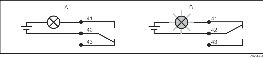
15 Recommended fail-safe switching for the alarm contact
