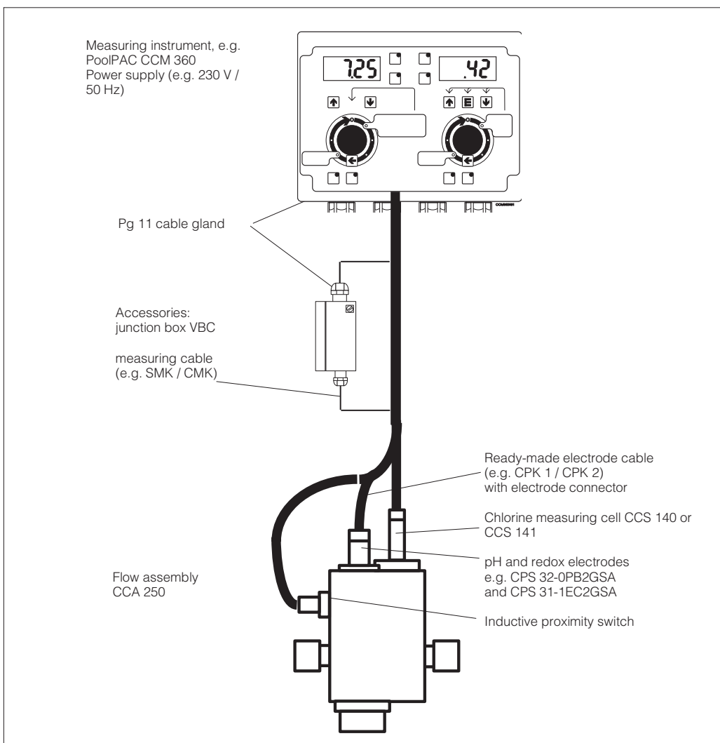
Fig. 1: Complete measuring system with flow assembly CCA 250, a measuring instrument, e.g. PoolPAC CCM 360, and junction box VBC
