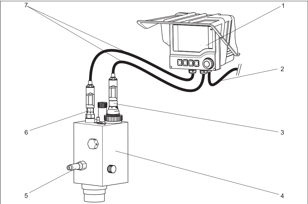
Fig. 3: Measuring system 1 Transmitter Liquiline M CM44 with weather protection cover 2 Supply line of the transmitter 3 Chlorine sensor CCS142D 4 Flowfit CCA250 5 Assembly inlet (outlet at backside, not to be seen in figure) 6 pH-Sensor 7 Measuring cable CYK10
