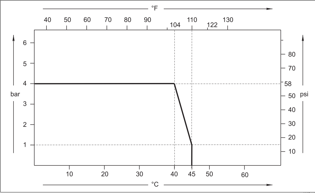
Fig. 6: Temperature-Pressure diagram
