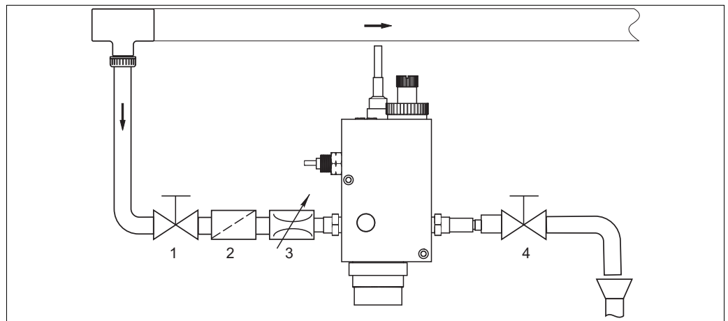
Fig. 5: Installation example with open outlet
