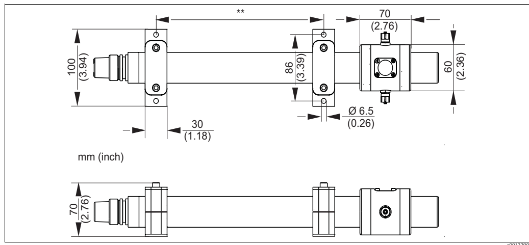
Fig. 13: Dimensions
