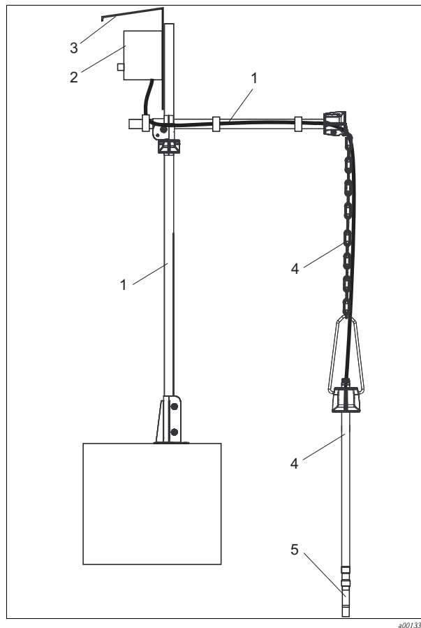
Fig. 4: Measuring system with immersion assembly (example)
