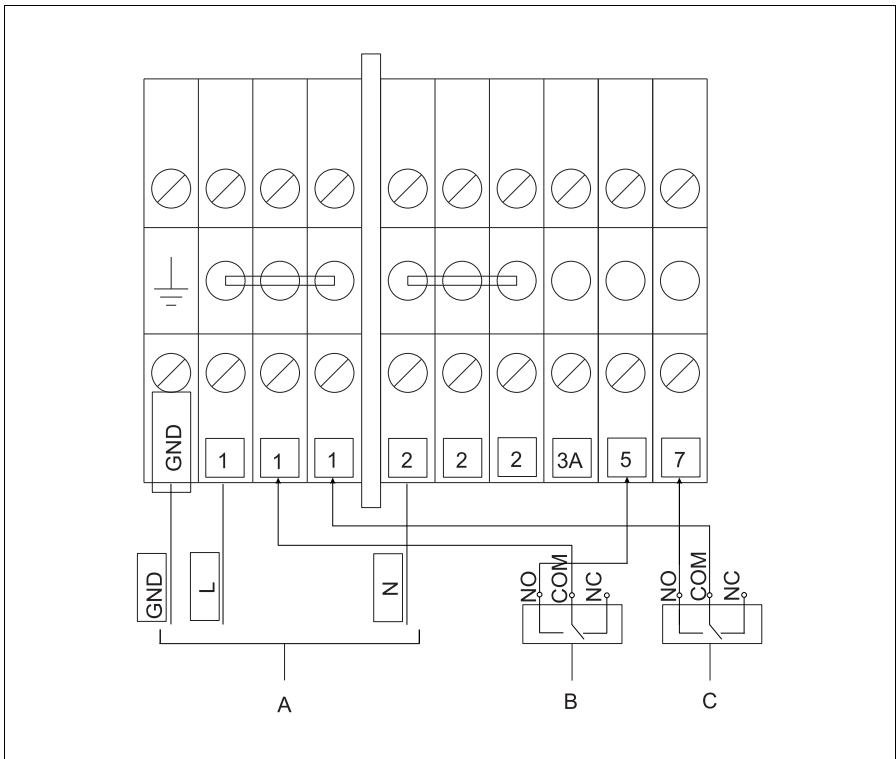
Fig. 7: Compressor point to point wiring diagram
