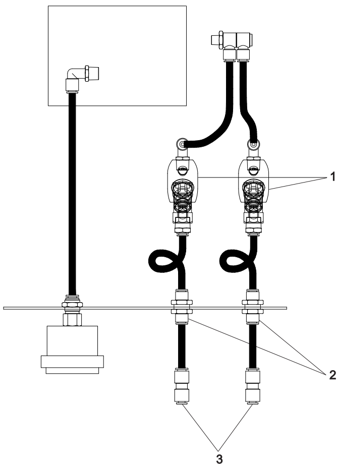
Fig. 3: Sensor installation - Connections
