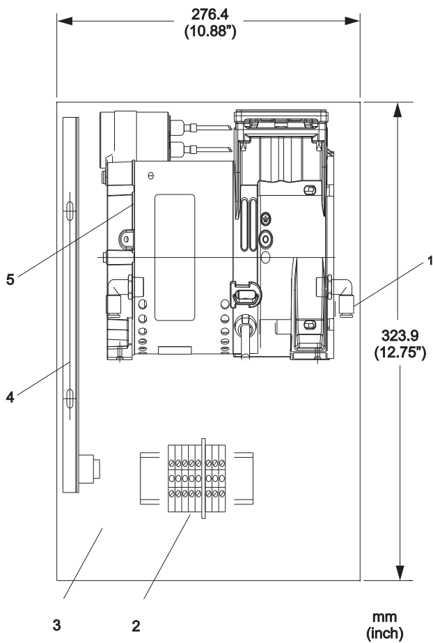
Fig. 1: Sensor installation - Front view 1 Fitting Bulkhead, 8 mm quick connect 2 Terminal strip 3 Sub panel 4 Heater 5 Air compressor
