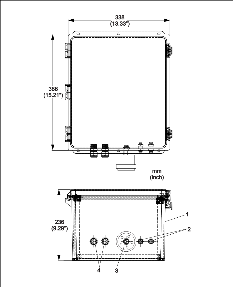
Fig. 5: Enclosure Detail
