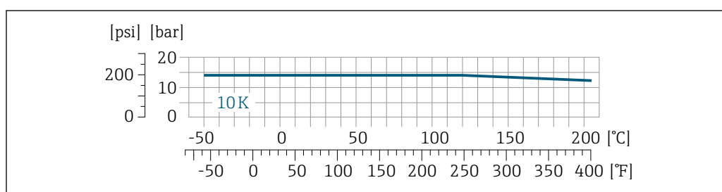
24 With flange material: 1.4539 (904L); lap joint flanges (not wetted): 1.4404 (316/316L)
