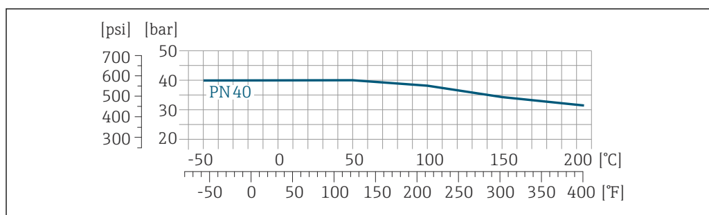
22 With flange material: 1.4539 (904L), Alloy C22; lap joint flanges (not wetted) 1.4404 (316/316L)
