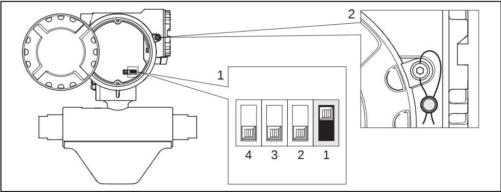
Switch locked
