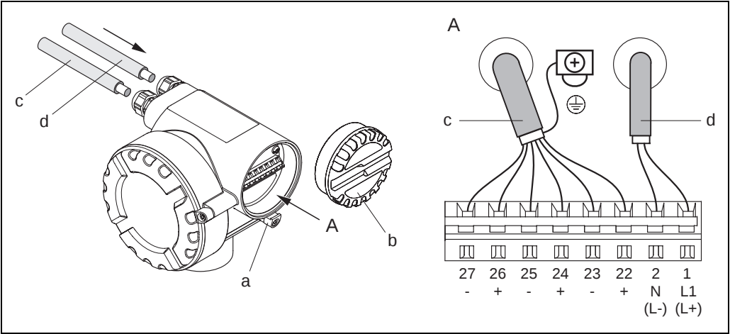
Connecting the transmitter, cable cross-section: max. 2.5 mm² (14 AWG)
