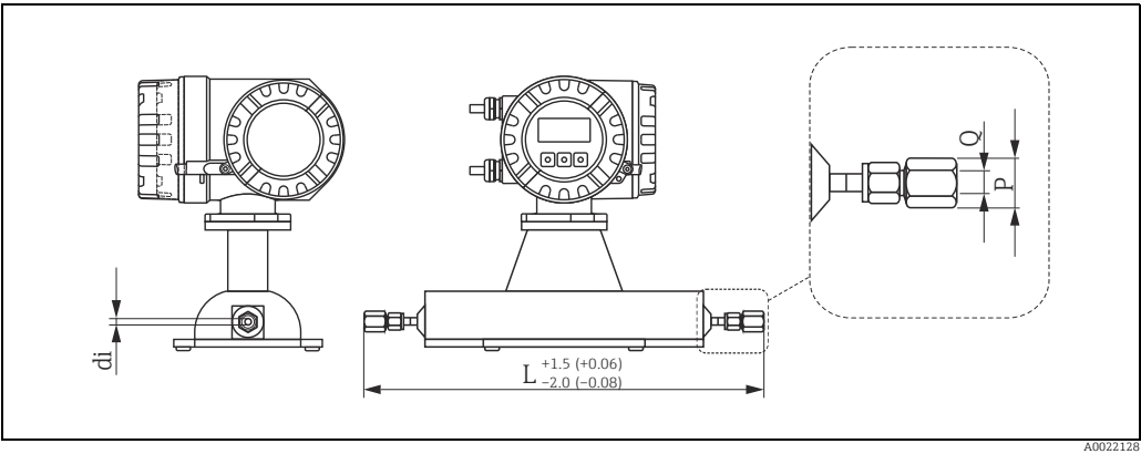
4-VCO-4 coupling with mounting kit: NPTF, 1/4"
