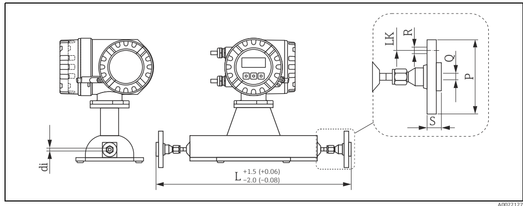
4-VCO-4 coupling with mounting kit DN 15 flange according to EN 1092-1 (DIN 2501), PN 40: 1.4539 (904L); Alloy C22
