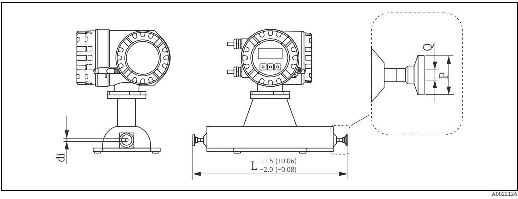
Tri-Clamp 1/2", DIN 11866 line C, 3A (welded)
