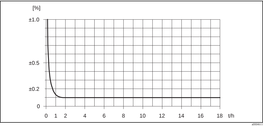
Max. measured error in % o.r. (example: Promass 83I / DN 25)
