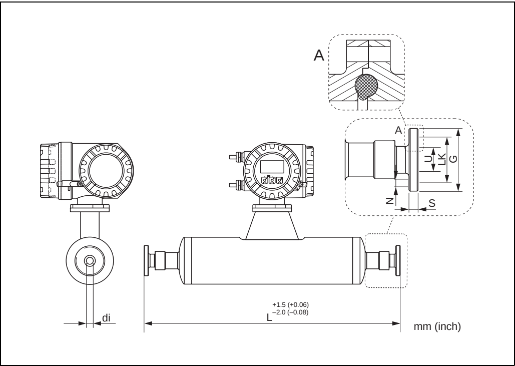
DIN 11864-2 Form A (flat flange with groove)
