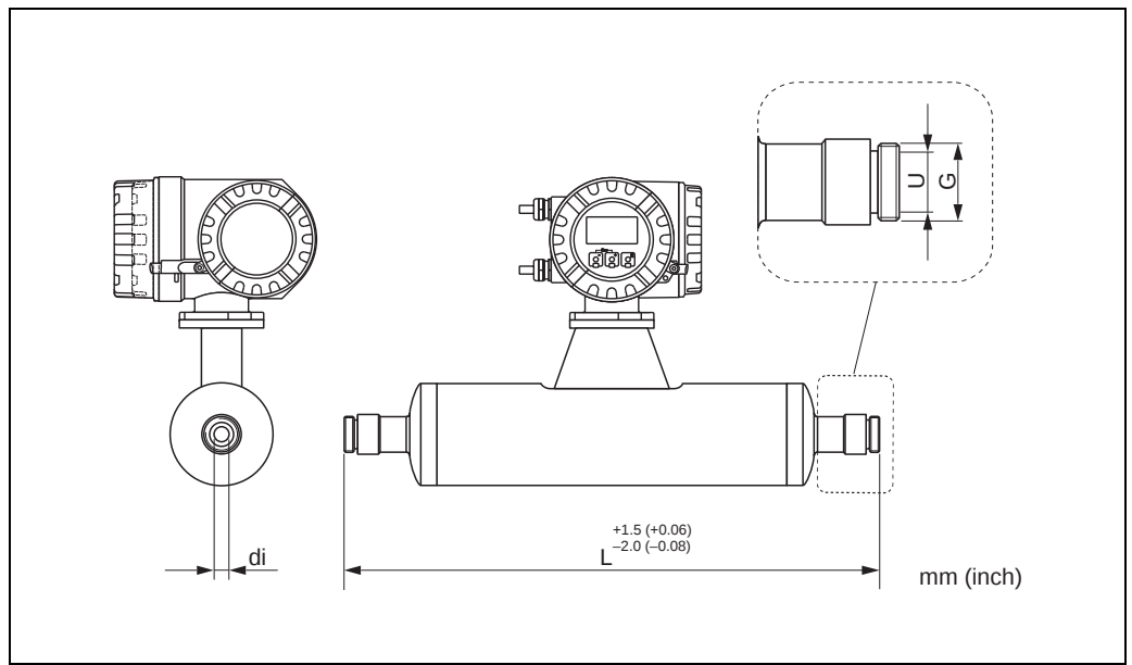
Threaded hygienic connection SMS 1145 / 3 version 1) ; Titanium
