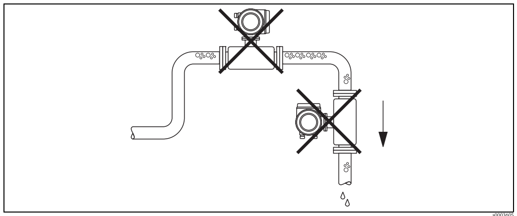
Mounting location
