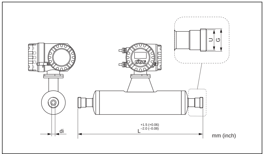
Threaded hygienic connection DIN 11851 / 3A version 1) : Titanium
