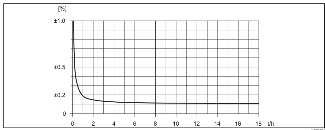
Max. measured error in % of measured value (example: Promass 83 F / DN 25)
