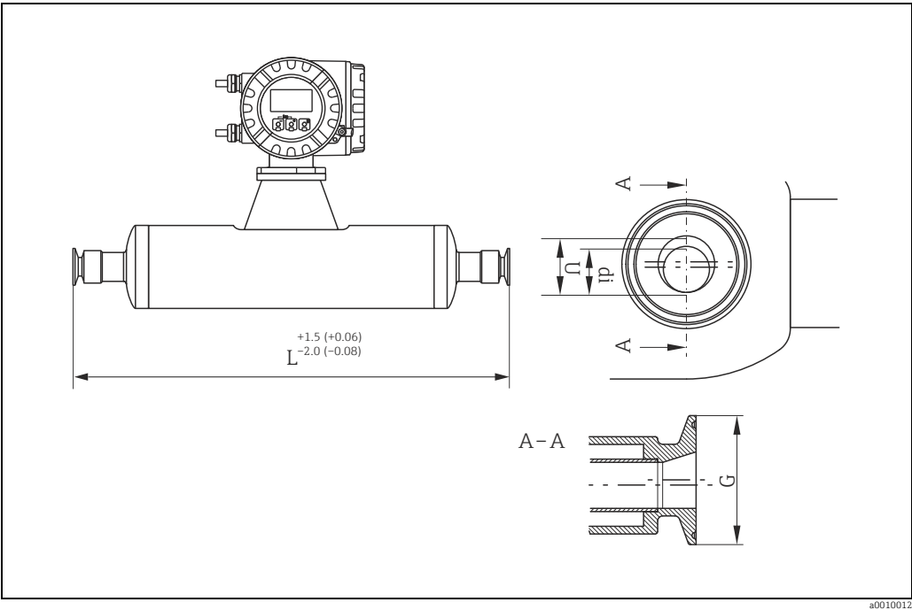
Tri-Clamp eccentric, DIN 11866 line C
