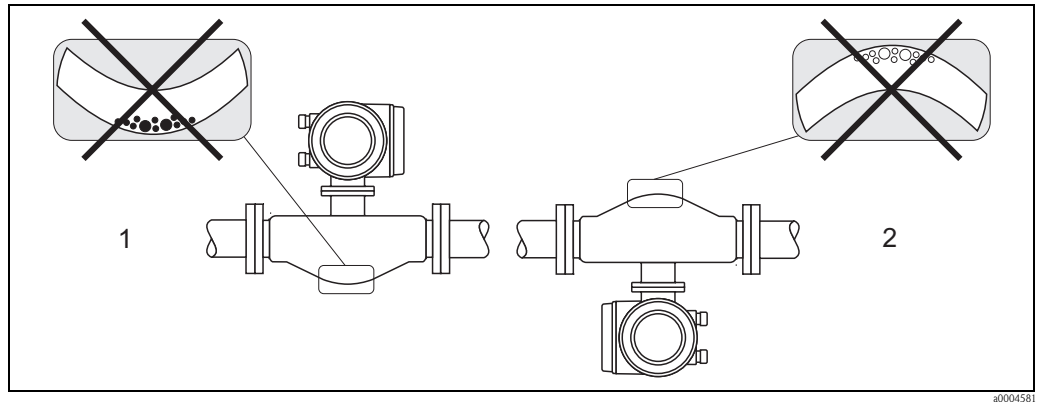
Horizontal installation for sensors with curved measuring tube
