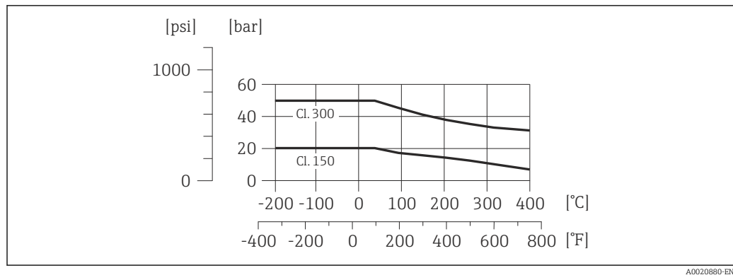
17 Process connection material: stainless steel, multiple certifications, 1.4404 (F316, F316L)
