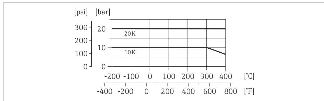
18 Process connection material: stainless steel, multiple certifications, 1.4404 (F316, F316L)
