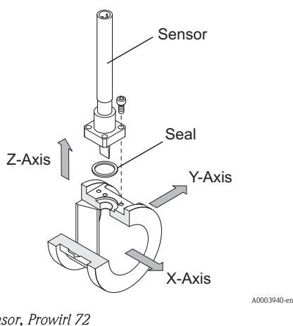
DSC sensor, Prowirl 72
