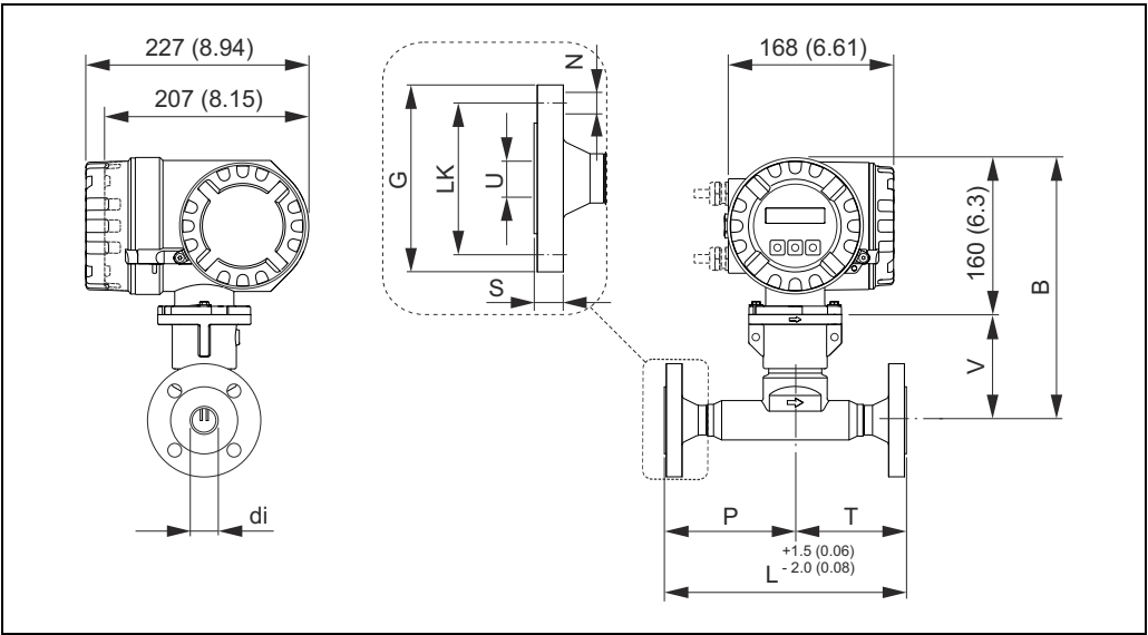
t-mass 65F: Flange connections as per ASME
