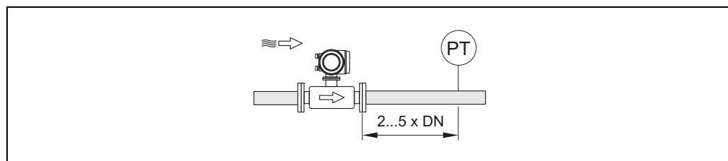
Installing a pressure measuring point (PT = pressure transmitter)
