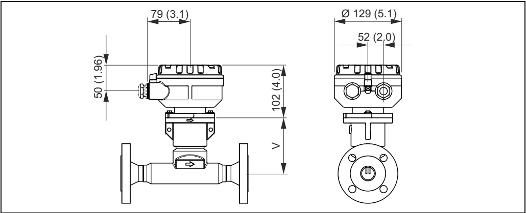
Engineering unit mm (in); dimensions "V": → 📄 31 and → 📄 33
