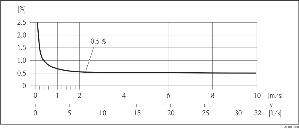
7 Maximum measured error in % o.r.
