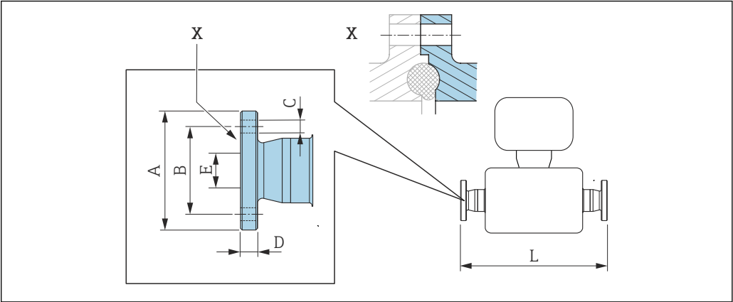
20 Detail X: Asymmetrical process connection; the part shown in gray is provided by the supplier.
