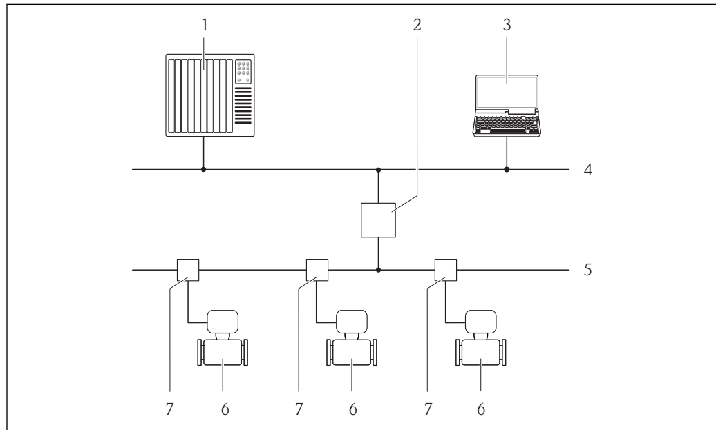
26 Options for remote operation via PROFIBUS PA network
