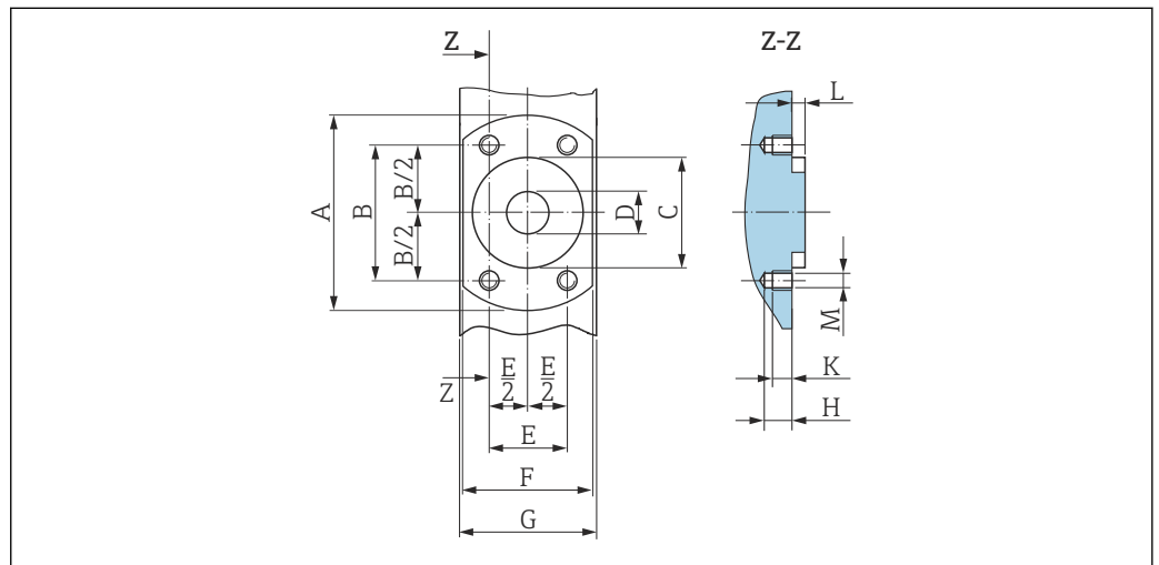
21 Front view without process connections
