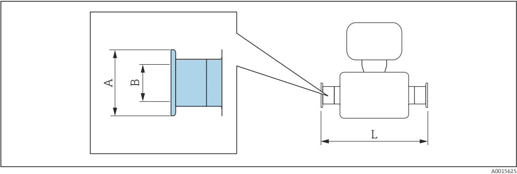
22 Hygienic clamp adapter connection suitable for pipes with connection according to ASME BPE (reduction)
