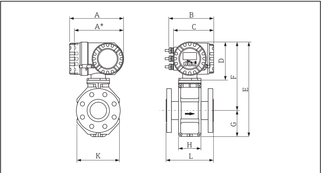
Dimensions (SI units)
