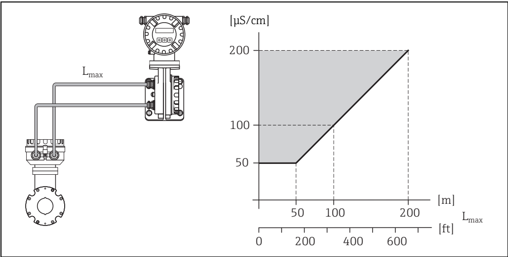
Permitted length of connecting cable for remote version - The area shaded gray marks the permitted range - Length of connecting cable L_{max} - Fluid conductivity in [ \mu\text{S}/\text{cm} ]
