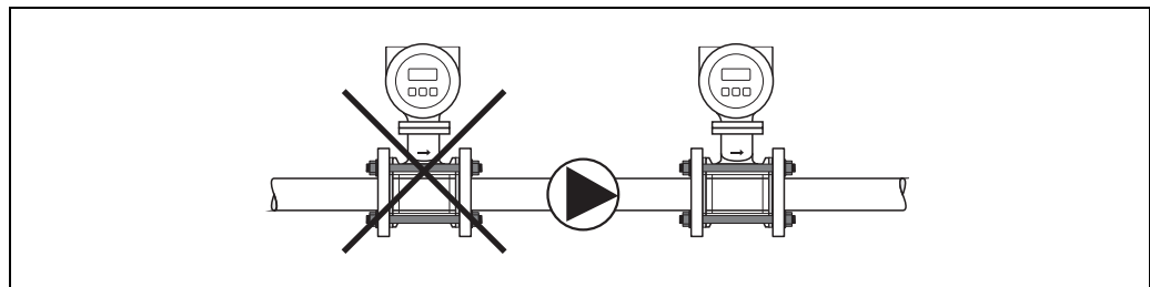
Installing the device with a pump
