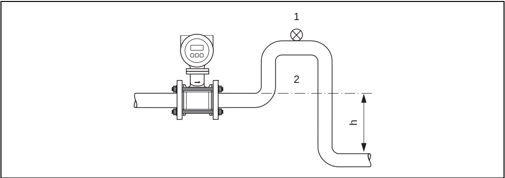
Installation measures for down pipes
