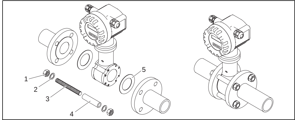
Mounting the sensor
